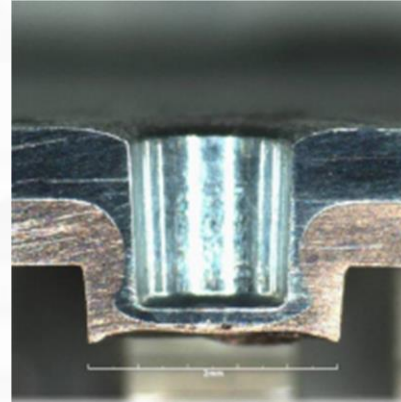
Clinching
